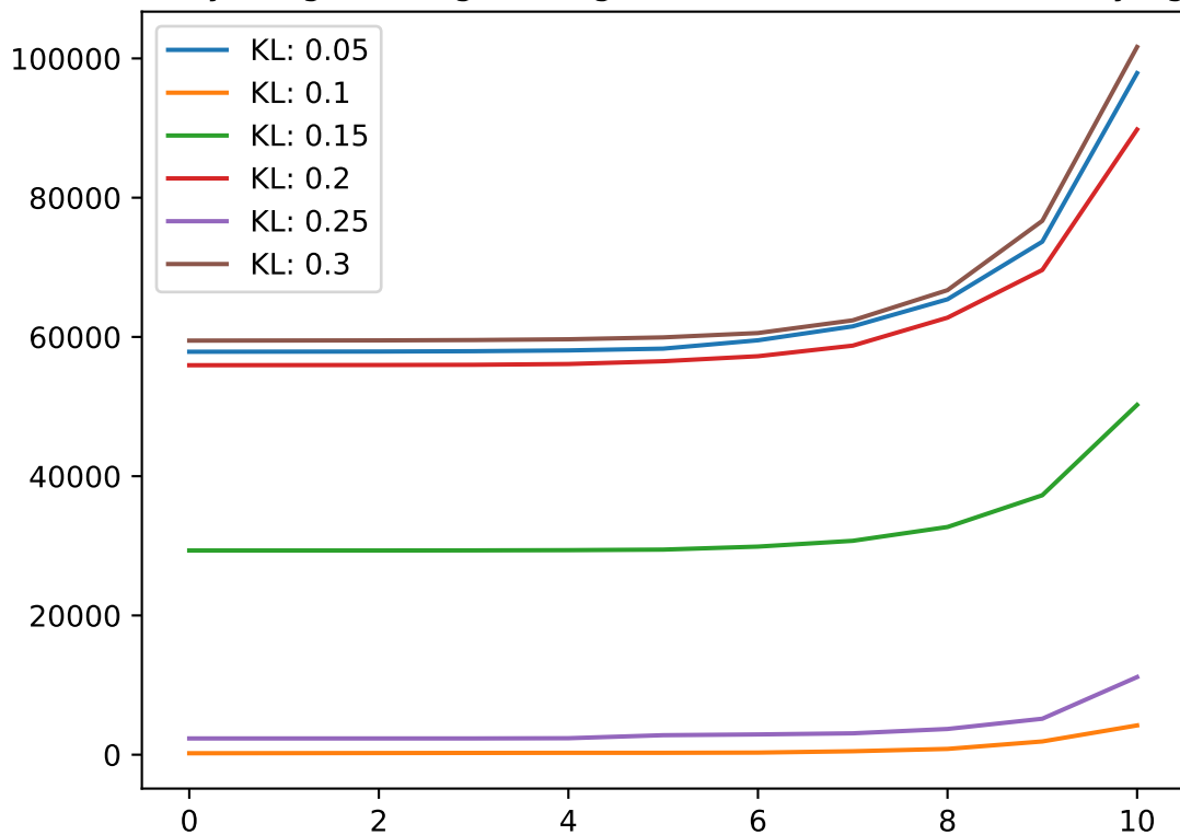
Memory usage of LogisticRegression for moon data of varying KL
